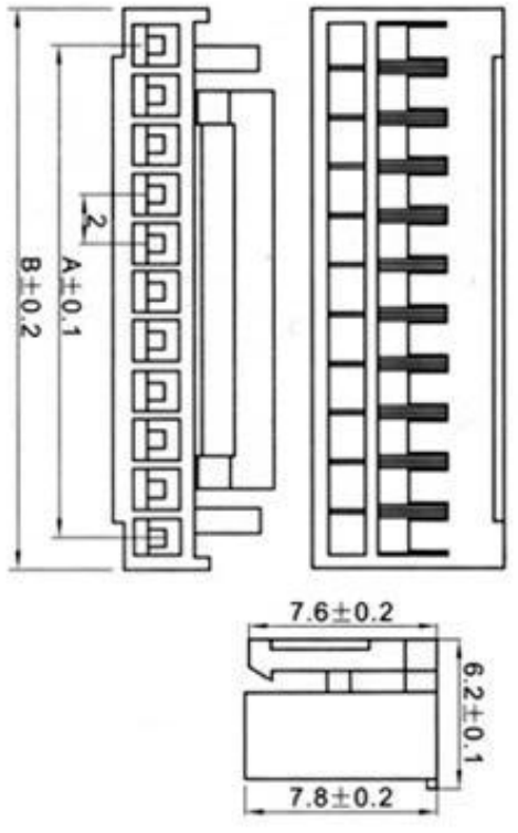
Housing
